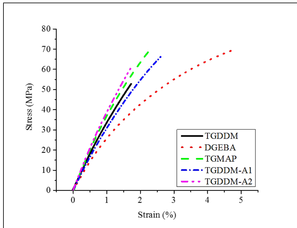
Figure 4. Representative stress – strain curves of tensile tests using macroscopic specimens
