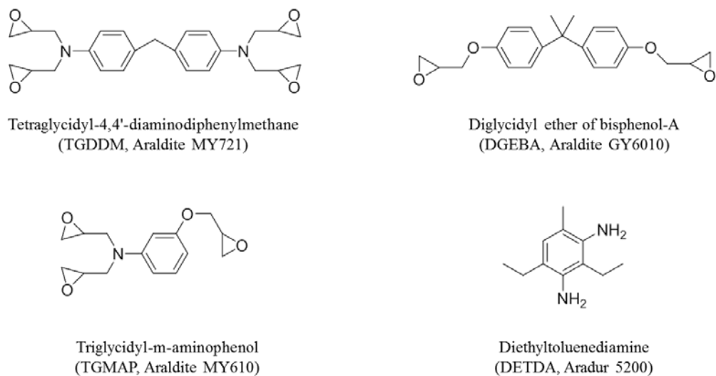
Figure 1. Epoxy compounds and curing agent used in this study
