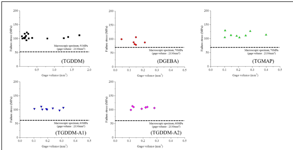
Figure 8. Failure stress against gage volume of specimens for each resin system
