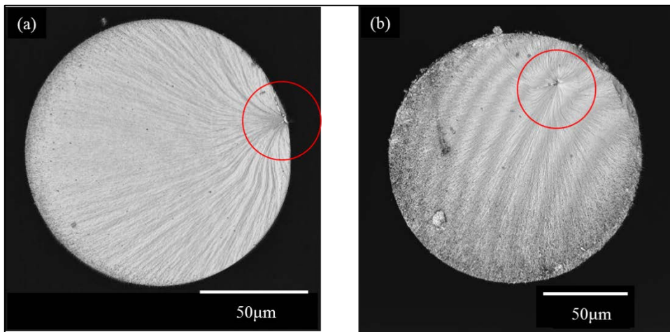
Figure 11. Fracture surfaces of epoxy fiber specimens after tensile test; (a) Surface initiation failure (b) Internal initiation failure
