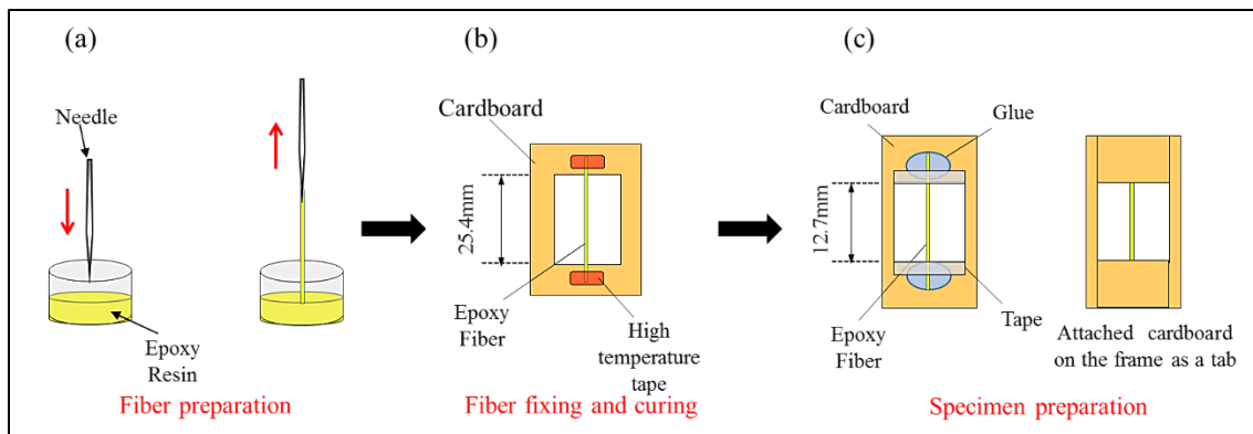
Figure 2. Preparation process of epoxy resin micro-fiber specimens
