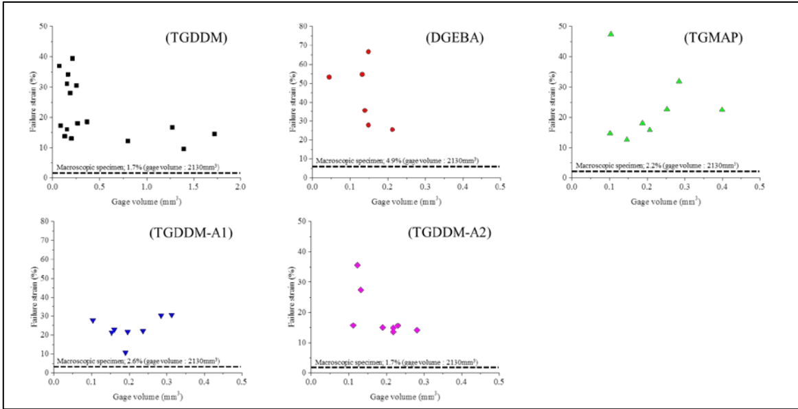
Figure 10. Failure strain against gage volume of specimens for each resin system
