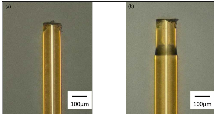
Figure 12. Side view of tensile failure location of epoxy fiber specimens (a) Failure without necking (b) Failure with necking
