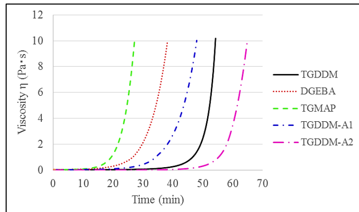
Figure 3. Isothermal viscosity-time curve for epoxy resin systems at 130°C
