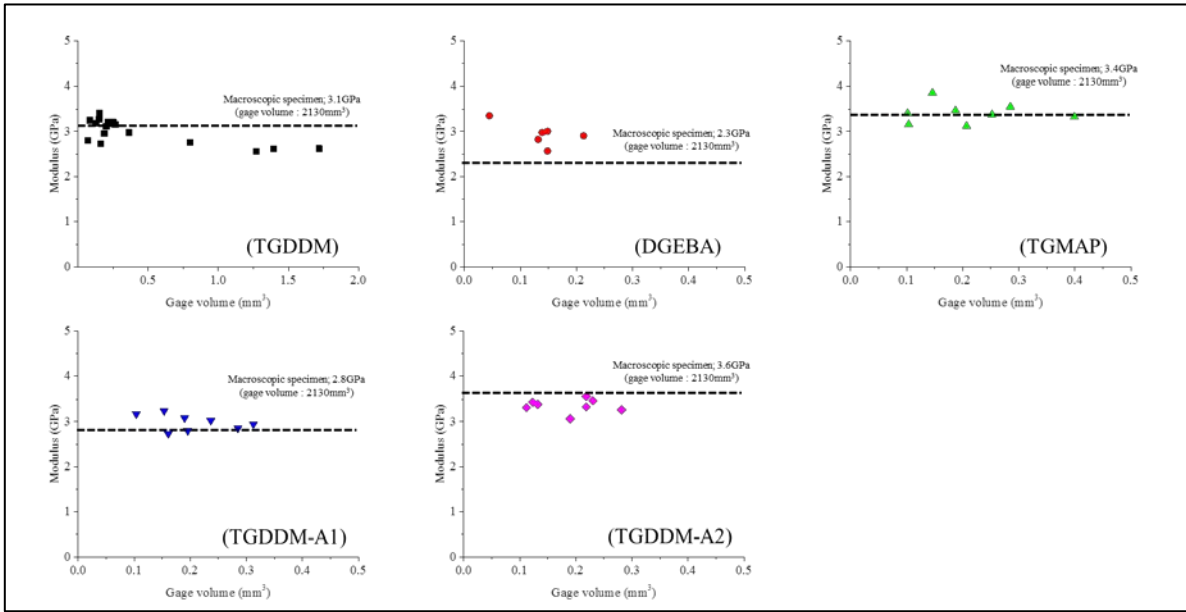
Figure 9. Young's modulus against gage volume of specimens for each resin system
