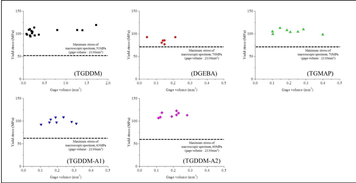
Figure 7. Yield stress against gage volume of specimens for each resin system
