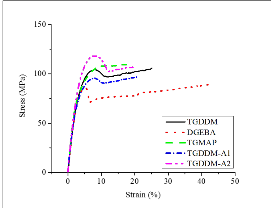
Figure 5. Representative stress – strain curves of tensile tests using epoxy micro-fiber specimens
