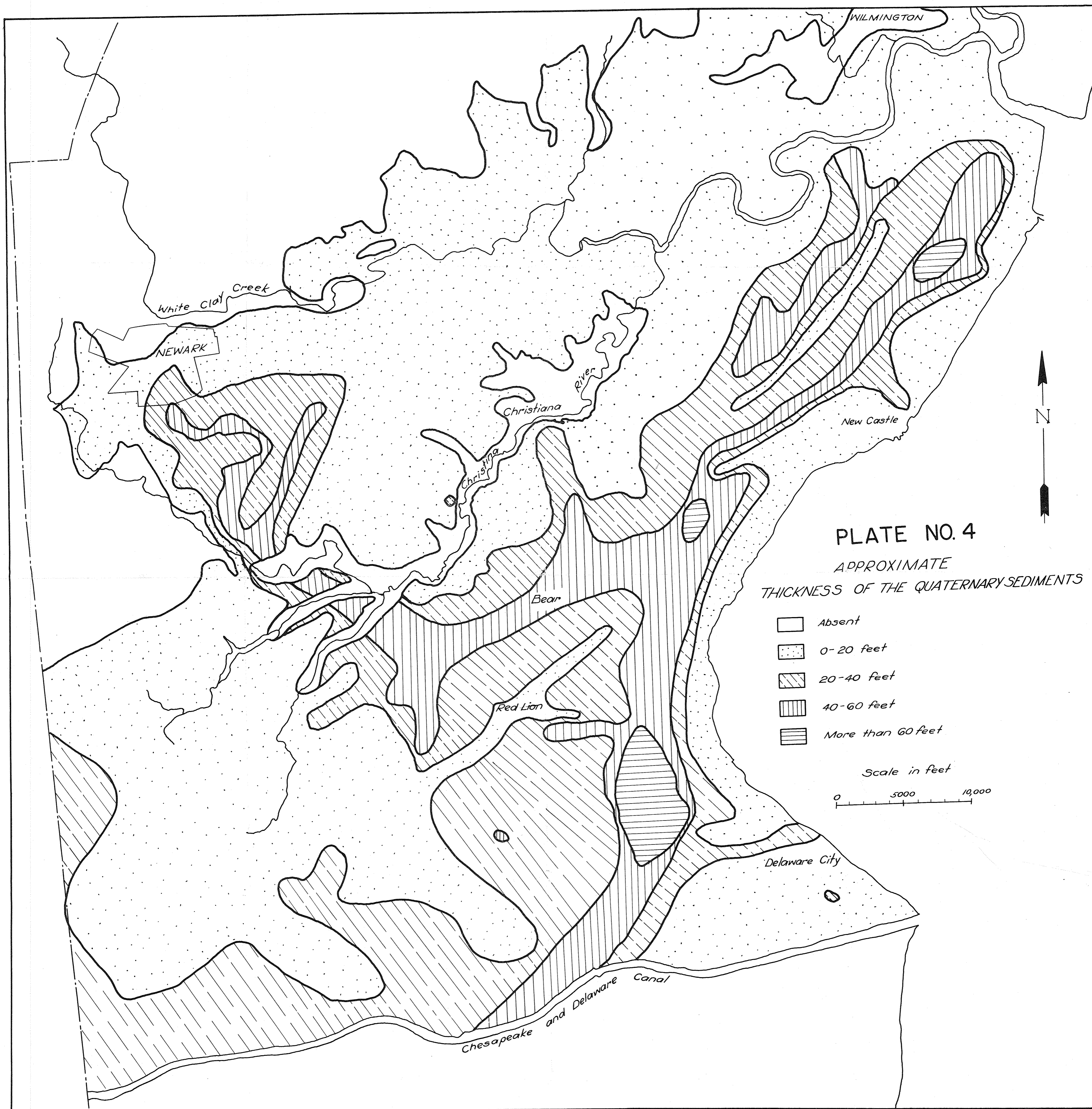
Plate 4. Approximate thickness of Quaternary sediments.
