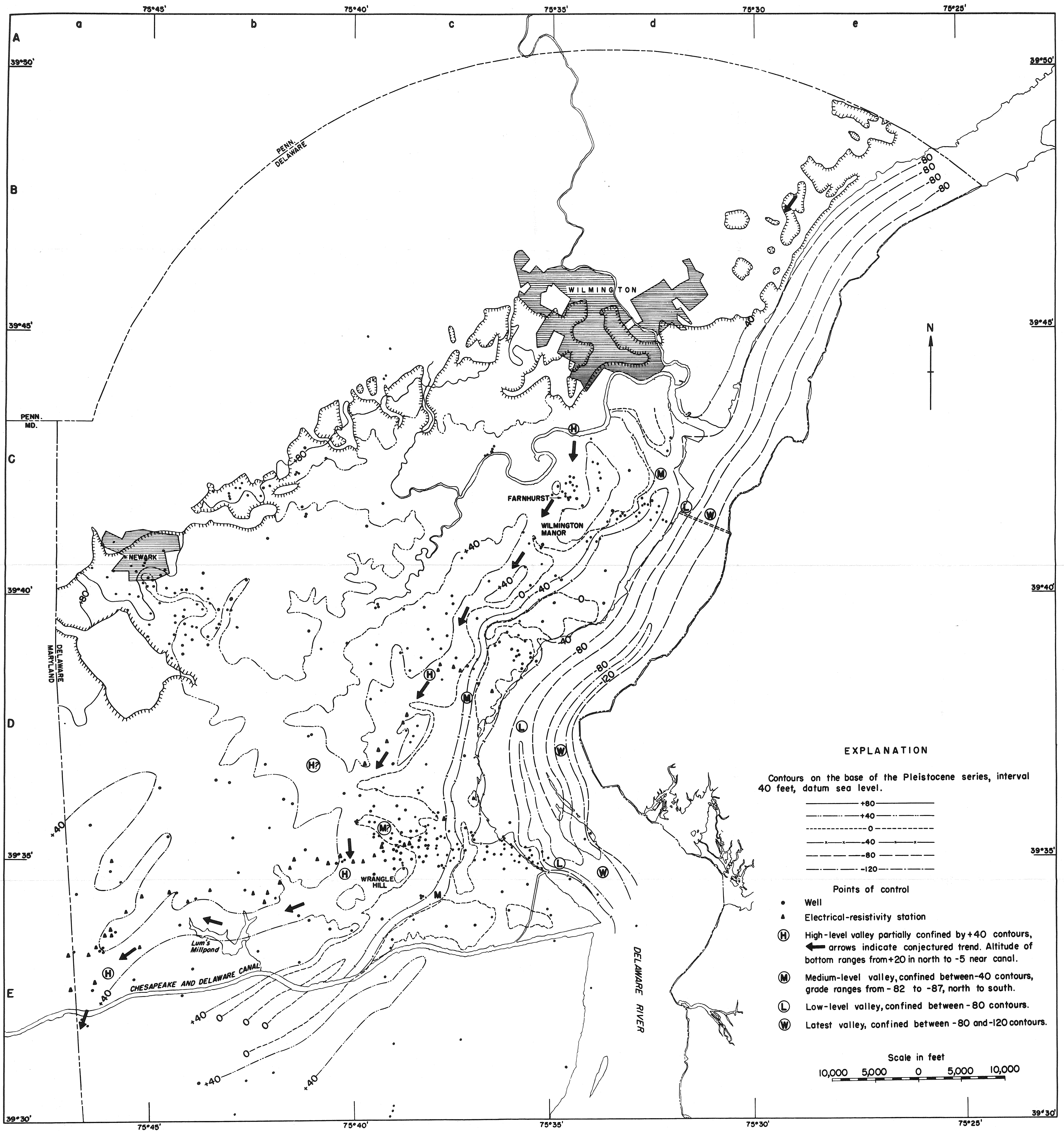
Plate 3. Map of base of Pleistocene series.
