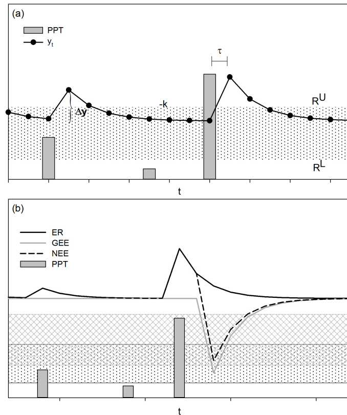
Figure A1. The threshold-delay model (Ogle and Reynolds, 2004). (a) The magnitude of the increase in the response variable ( \Delta y , e.g., carbon flux, y_t ) is determined by the size of the PPT event and by the previous state of the response variable. The decreasing rate of the response following the stimulus is denoted by -k . The low PPT threshold ( R^L ) indicates the minimum size of the PPT event to stimulate a response, and the upper PPT threshold ( R^U ) indicates PPT events that do not cause additional increments in the response variable. The time interval between the stimulus and the response is described by \tau . (b) The response of the net ecosystem exchange (NEE), which is the balance between the gross ecosystem exchange (GEE) and ecosystem respiration (ER), varies in response to changes in GEE and ER. According to the T-D model, GEE and ER have different PPT thresholds (dotted band and mesh stand for effective PPT event size for ER and GEE, respectively), with ER responding to smaller-sized PPT events than GEE; therefore, small PPT events favor C release, whereas large PPT events stimulate net C uptake by the ecosystem. Differences in time responses between soil microorganisms and plants to soil wet-up led GEE and ER to differ in time delays ( \tau ), with shorter time delays for ER than GEE (Huxman et al., 2004a). The hypothetical curve for NEE and its components were calculated, introducing arbitrary parameters in the T-D model equations of Ogle and Reynolds (2004).
