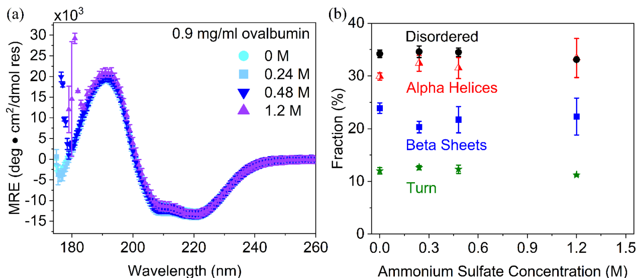
FIGURE S3. A: CD data shown as the mean residue ellipticity (MRE) for 0.9 mg/mL ovalbumin at room temperature with varying AS concentrations, color-coded as labeled. Error bars are standard errors in MRE based on three averaged measurements per condition. B: Secondary structure fractions determined from deconvolution of circular dichroism data using the CONTINLL algorithm in Dichroweb, and Reference data set SP175 5-7 . The NRMSD for the fits to the 0, 0.24, 0.48, and 1.2 M AS solutions were 0.021, 0.024, 0.023, and 0.048, respectively. The error bars are standard errors between three successive deconvolutions at each condition.
