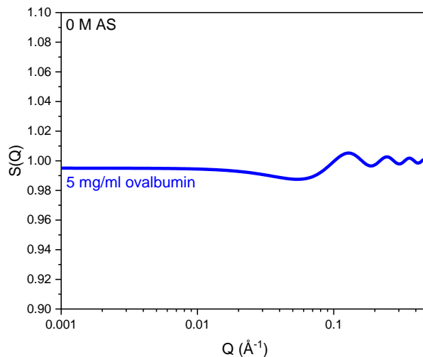
FIGURE S5. Structure factor profile calculated from b_2^* for AS-free 5 mg/ml ovalbumin, using the master curve equation to validate the initial assumption of no significant protein-protein interaction contributions to the corresponding SAXS data. The contribution from the structure factor to the scattering intensities are < 1\% across the fit range ( 0.01 \text{ \AA}^{-1} < Q < 0.4 \text{ \AA}^{-1} ).
