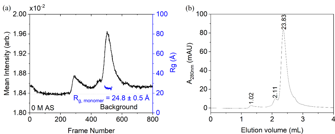
FIGURE S1. A: X-ray scattered intensities for the SAXS-elution profile of AS-free ovalbumin solution in 5 mM phosphate buffer pD 7 (injection of 50 \mu\text{L} of protein solution at 15 mg/mL). The dashed line shows the background signal from buffer. The main peak radius of gyration R_g (blue) were calculated using liquid chromatography (LC) series analysis available in BioXTas RAW 1,2 . The R_g of 24.8 \text{\AA} fitted to the main peak is consistent with the monomer as the dominant species in solution. The average data for the main peak was used to produce a 1D scattering profile, which was then fitted to determine the reduced second virial coefficient b_2^* . B: Corresponding UV absorption profile for the 4 mL elution measurement. The monomer peak (eluted at 2.5 mL) represents \approx 88\% of the total area of the absorbance intensity.
