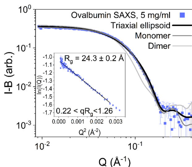
FIGURE S4. Ambient pressure SAXS data measured for 5 mg/mL ovalbumin solution in 5 mM sodium phosphate buffer pD 7 at room temperature. The buffer contributions have been subtracted from the data. The triaxial ellipsoid best-fit curve (black) is shown overlapping with the data (blue) and theoretical scattering calculated from the monomer (gray) and dimer (light gray) crystal structure 10 . Inset: Guinier fit to the low Q data, for radius of gyration determination, shown in black. Error bars arise from experimental counting statistics.
