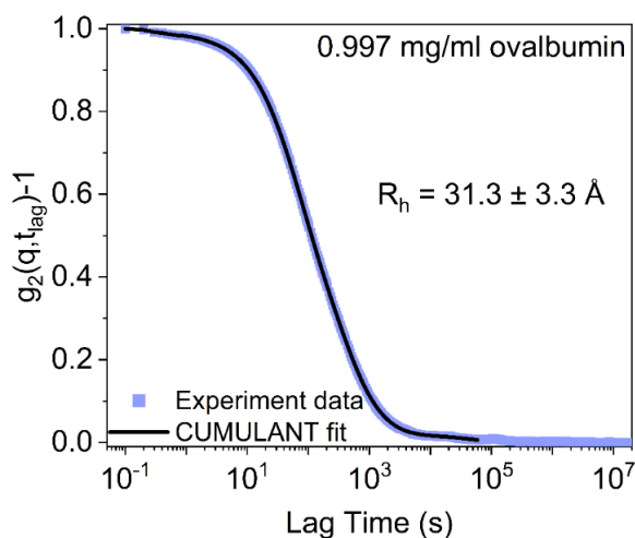
FIGURE S2: Cumulant fit to g_2(q, t_{lag}) - 1 for AS-free 0.997 mg/ml ovalbumin solution in 5 mM deuterated phosphate buffer (pD 7). The DLS data was collected at a scattering angle 90^\circ , at 23^\circ\text{C} . The average hydrodynamic radius was determined to be 31.3 \text{ \AA} , yielding R_g/R_h \approx 0.776 , close to the expected average ratio of 0.775 for globular proteins 4 .
