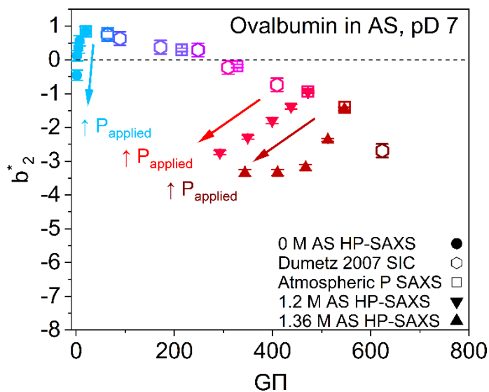
FIGURE S10. Ovalbumin b_2^* as a function of the osmotic pressure contributions, for data collected at various AS concentrations and applied hydrostatic pressures ( G = 5.94 ). Applied hydrostatic pressures for the three HP-SAXS series (blue, 0 M AS; red, 1.2 M AS; dark red, 1.36 M AS) are, in the direction of the arrows: 10, 98, 195, 265, 350 MPa. The hydrostatic pressure for all other points is atmospheric ( \approx 0.1 MPa).
