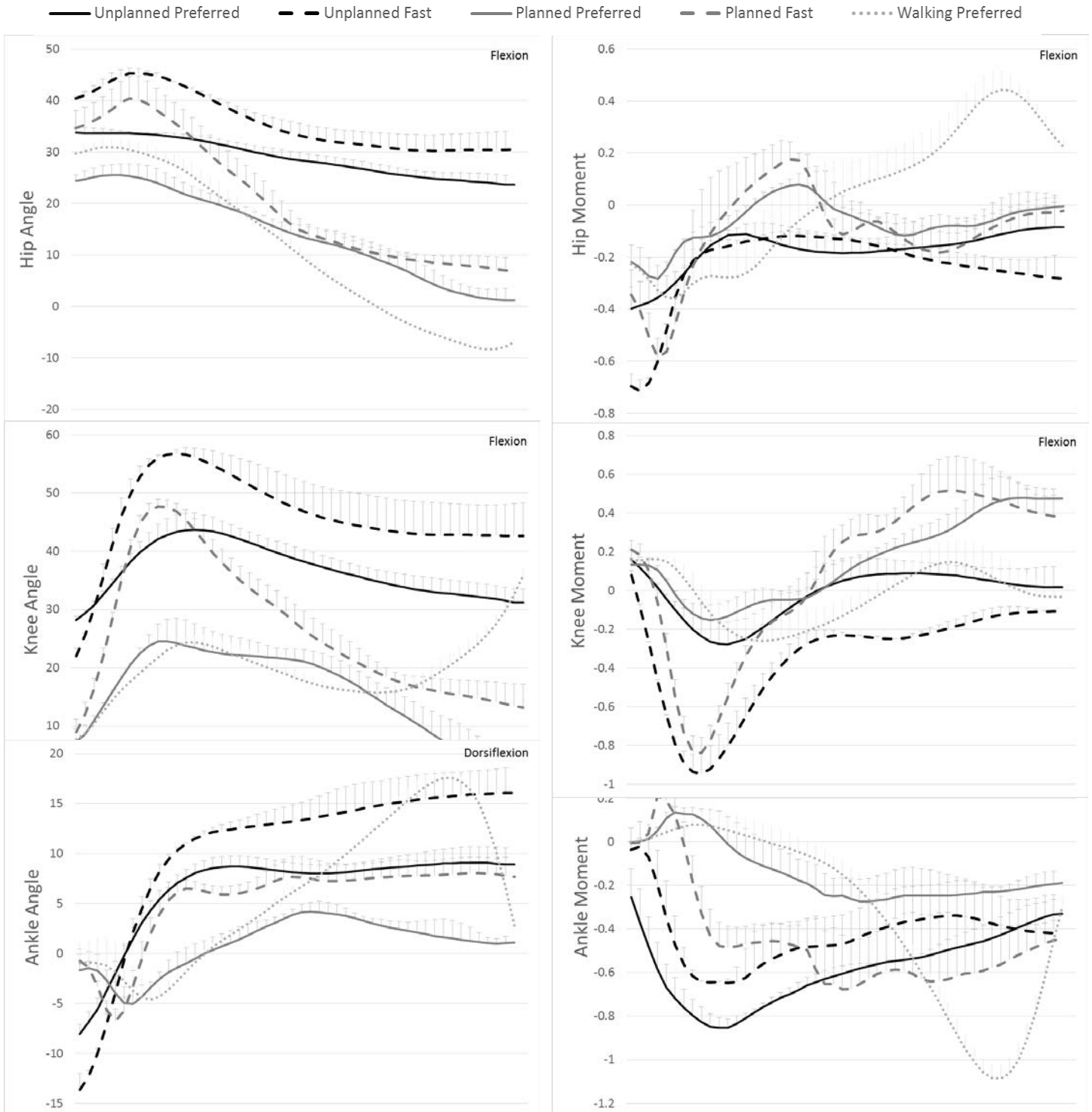
Figure 2. Representative joint angles and internal joint moments during the stop stance phase for the lead leg during all stopping conditions and stance phase during preferred speed walking. Graphs show data for each condition for a representative subject. The start of the graph represents terminal foot contact (or foot contact, for walking), while the end represents stable stop position (or toe-off, for walking). Data from each stance phase was time normalized for comparison.
