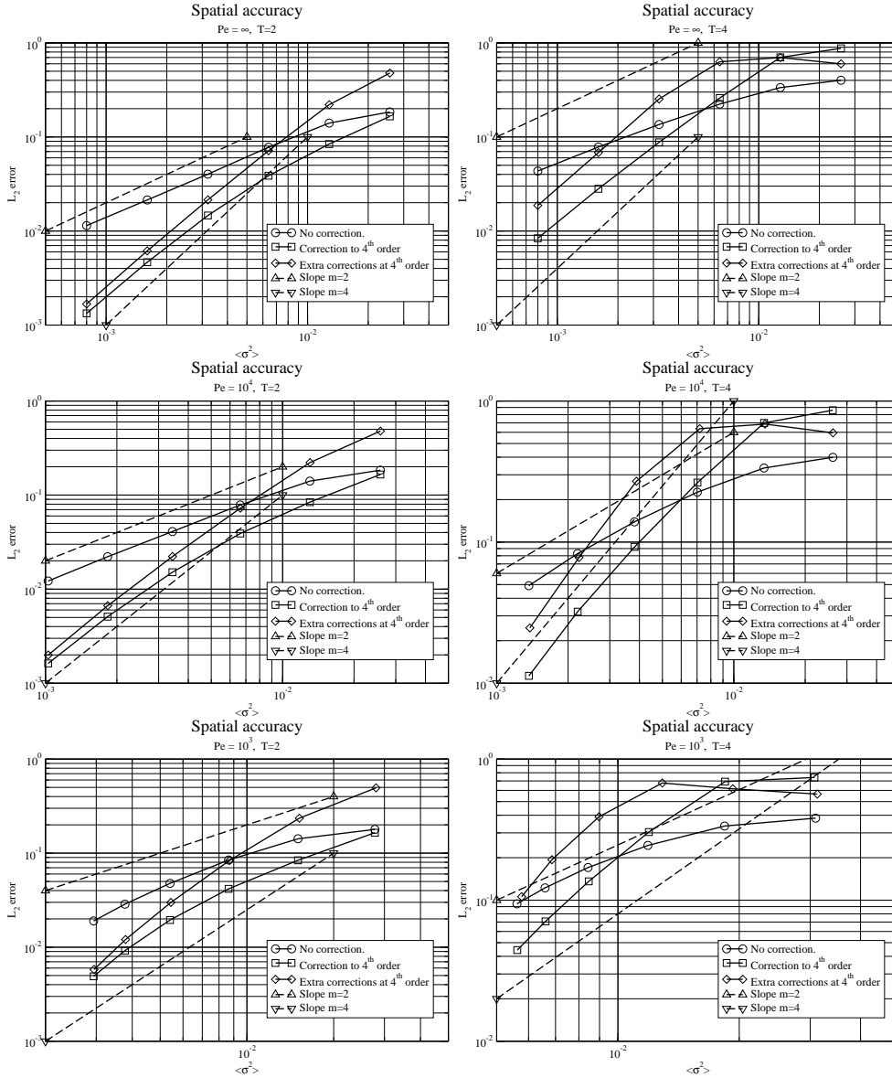
FIG. 7.2. Improved spatial convergence properties for the convection diffusion equations at three different Peclét numbers. The characteristic core width \langle \sigma^2 \rangle is the scalar weighted average core width at T = 2 and T = 4 , respectively. These correspond to the field after one half and one full turnover time. These graphs demonstrate the improved spatial accuracy when using corrected velocity fields ( \square 's) compared to using centroid velocity data ( \circ 's). The third curve ( \diamond 's) is data when some of the fourth order terms are eliminated using (5.4). It is impossible to eliminate all of them using elliptical Gaussian basis functions with the velocity correction technique proposed in this paper.
