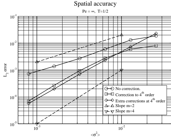
FIG. 7.3. Slight advantages in partial error cancellation for short times. We see that canceling two of the fourth order terms offers some improvement. However, the advantages are slight and disappear for larger T .
