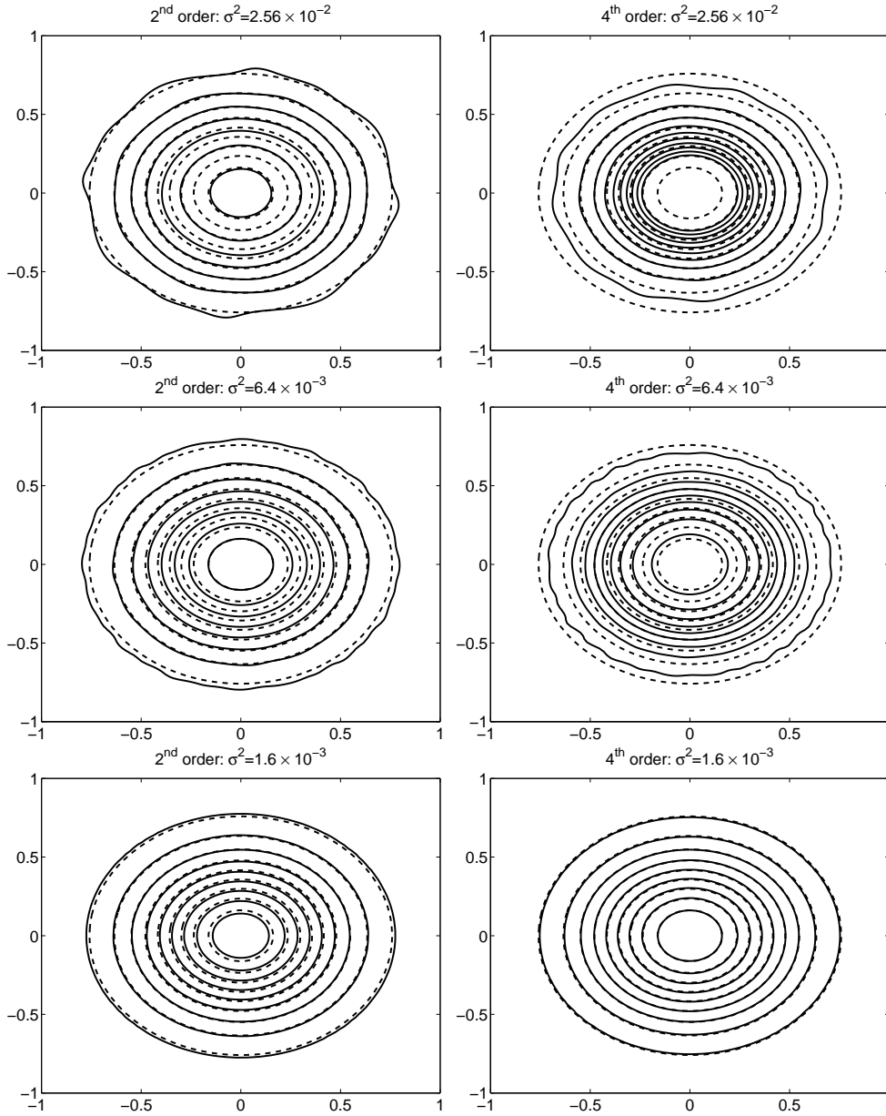
FIG. 7.5. Comparison of scalar fields with second- and fourth-order schemes at Pe = \infty . The exact solution (dashed) is shown together with the computed (solid) contours. The second-order results are in the left column and the fourth-order results are in the right. Each row represents different core sizes, diminishing from top to bottom. The contour increments are 0.4 scalar units.
