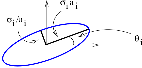
FIG. 3.1. A schematic diagram of an elliptical Gaussian basis function as defined in (3.5). The ellipse is representative of a single level set.
