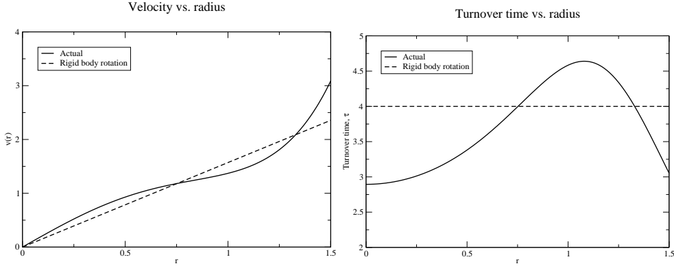
FIG. 7.1. Velocity and turnover time for the flow field described by \psi in (7.1) with \delta = \frac{1}{10} , c_1 = -\frac{7}{2} and c_2 = 3 . Rigid body rotation is shown for comparison.
