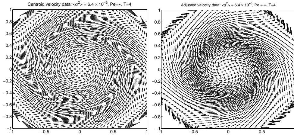
FIG. 7.4. Typical basis function positions at T = 4 . When using centroid data, basis functions follow streamline. However, the higher spatial order method need not do so. Similar behavior is seen for all experiments though to a lesser extent when \langle \sigma^2 \rangle is smaller. Blobs are shown as \times 's where the arm lengths are \frac{1}{5}\sigma_i a_i and \frac{1}{5}\frac{\sigma_i}{a_i} , and we see that aspect ratios vary considerably over the domain due to variations in the local shear. Contour lines of \hat{\rho} are superposed at intervals of 0.4, and the L_2 error for this choice of core size is about the same for both methods. On the left, the simulation uses centroid velocity data and the particle densities remain uniform. On the right, the simulation uses adjusted velocity data to achieve fourth-order accuracy. In this case, particles no longer follow the concentric streamlines, and density variations occur. In both plots, skinnier basis functions can have aspect ratios of 15 or more.
