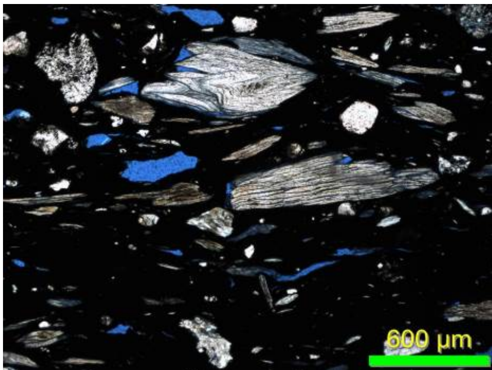
Figure 21. In thin sections of fired sherds, especially those fired below 1000°C, there is enhanced parting and splitting between layers of some of the talc particles that occurs with loss of water of hydration. These underfired talc particles are friable until fired at a temperature above 1000°C (C. L. Reedy).
