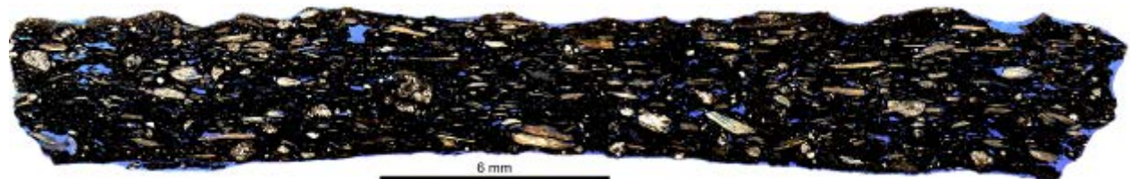
Figure 19. Scanned thin section of a second fired sherd which is thinner and has more elongated and aligned talc particles (2.8 – 4.5 aspect ratio versus the mean of 2.3 for Fig. 18) (C. L. Reedy).
