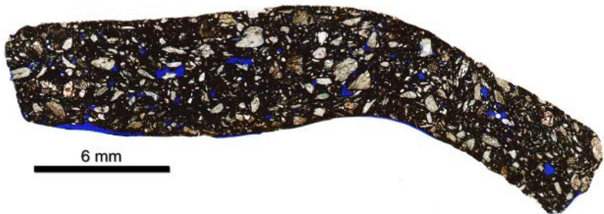
Figure 18. A scanned thin section from a fired sherd (C. L. Reedy).
