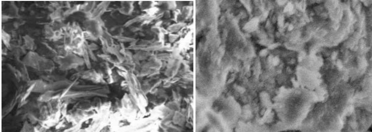
Figure 16. Microstructure of raw materials: Talc with sharp, angular, platy structure (left, 500x); clay with a wide range of poorly formed clay particles, 0.5-12 \mu (right, 8000x) (P. B. Vandiver).
