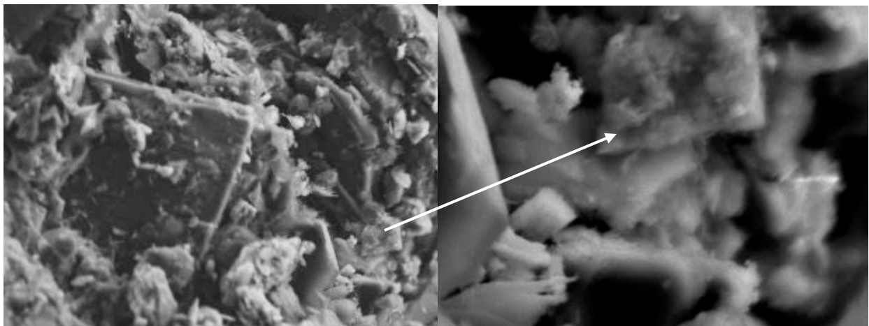
Figure 17. A fresh fractured surface from a serving plate exhibits a fired ceramic microstructure at 670x (left) and 10,000x (right). Edges of talc particles have begun to soften and to lose their angular crystalline shapes. The clay has begun to sinter to the talc particles and to lose surface definition when fired at the estimated firing temperature of about 1100°C. The square platy particle on the right is also present in the lower right of the image on the left. These images were taken of a fractured surface made parallel to the pot's surfaces in order to detect the alignment that occurred during fabrication. Compared to Fig. 17, right, significant alignment and increased fracture strength is attained by the application of shear force during fabrication (P. B. Vandiver).
