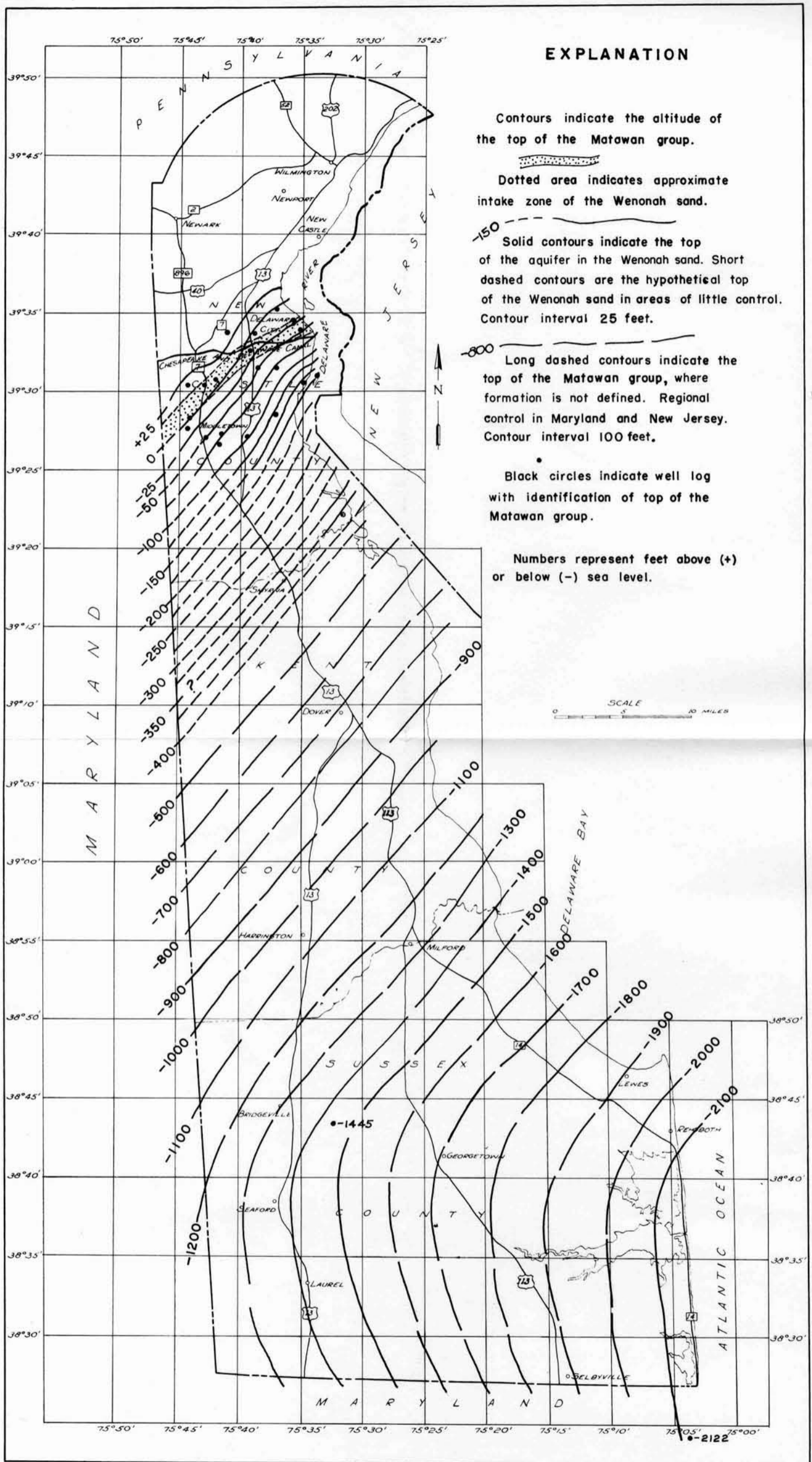
Plate 7.—Structure map of the top of the Matawan group and of the Wenonah sand.
