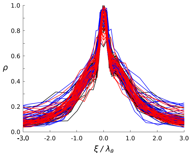
FIG. 8. Absolute value of the correlation maps, evaluated at the eddy-specific wall-distance y_{\text{MAX}} , where the eddy velocity profile has its maximum. Showing all profiles for the range m \in [5, 35] . \text{Re}_\tau = \{1310, 2430, 3810\} are shown in black, blue, and red, respectively.
