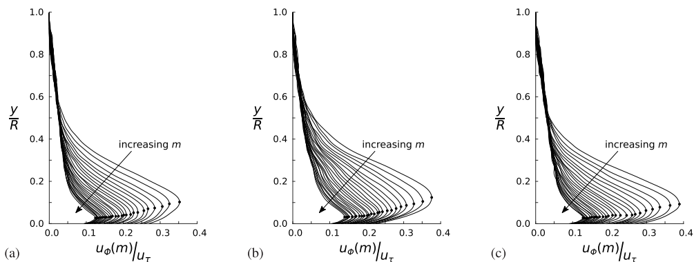
FIG. 3. The average eddy velocity profiles for all m \in [10, 35] . (a) \text{Re}_\tau = 1310 . (b) \text{Re}_\tau = 2430 . (c) \text{Re}_\tau = 3810 . The symbol \bullet marks the peak location for each eddy velocity profile.
