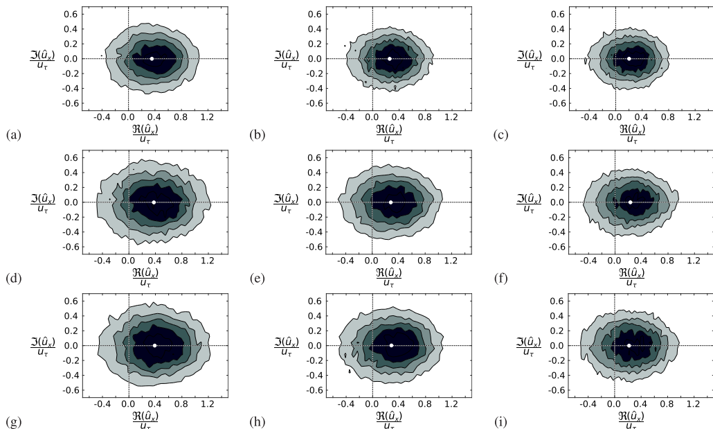
FIG. 4. PDFs of the streamwise velocity component u_x , evaluated at the peak eddy velocity location found in Fig. 3 (real and imaginary parts). The corresponding peak eddy velocity found in Fig. 3 is shown with a solid white circle. (a) Re_\tau = 1310 , m = 10 . (b) Re_\tau = 1310 , m = 15 . (c) Re_\tau = 1310 , m = 20 . (d) Re_\tau = 2430 , m = 10 . (e) Re_\tau = 2430 , m = 15 . (f) Re_\tau = 2430 , m = 20 . (g) Re_\tau = 3810 , m = 10 . (h) Re_\tau = 3810 , m = 15 . (i) Re_\tau = 3810 , m = 20 . Each PDF is scaled by its peak value and is shown with contour levels \{0.2, 0.4, 0.6, 0.8\} .
