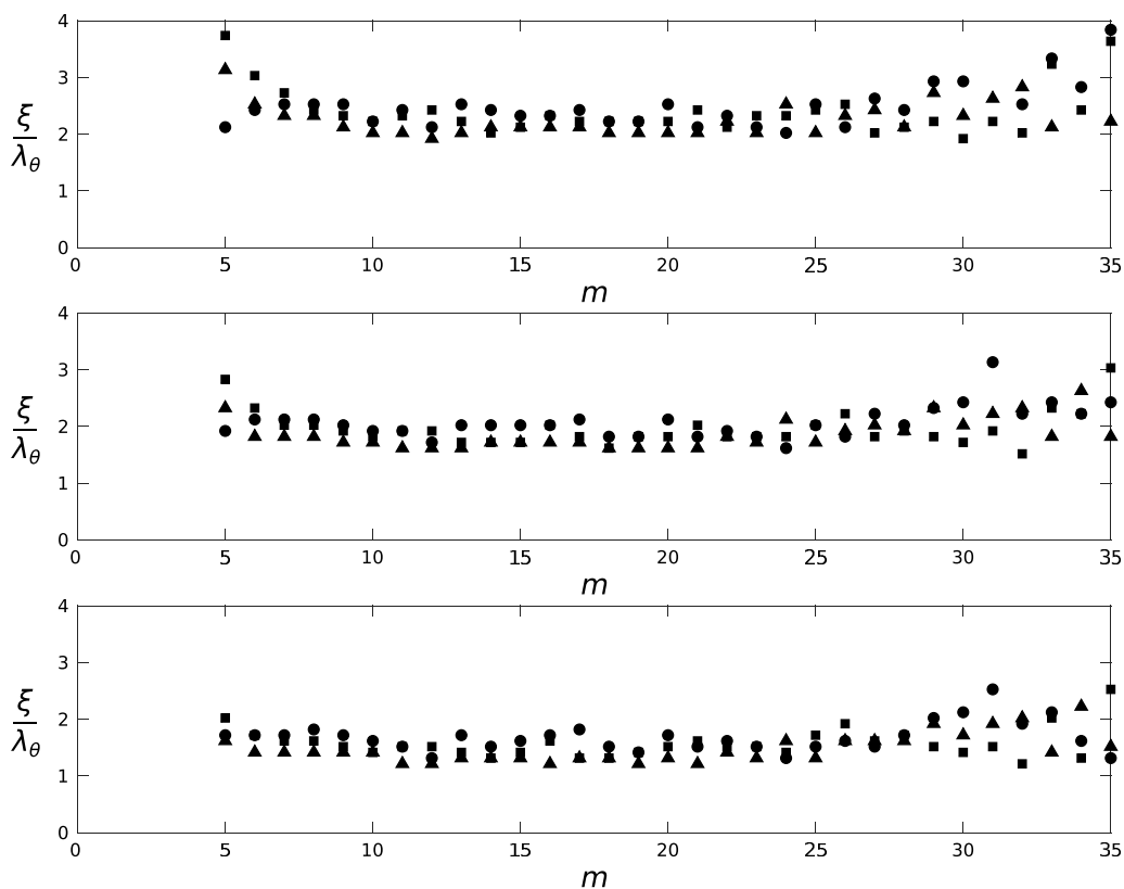
FIG. 9. Streamwise correlation lengths, evaluated from the profiles in Fig. 8. The considered thresholds are: (a) \rho = 0.08 , (b) 0.10 , (c) 0.12 . \blacktriangle \text{Re}_\tau = 1310 ; \blacksquare \text{Re}_\tau = 2430 ; \bullet \text{Re}_\tau = 3810 .
