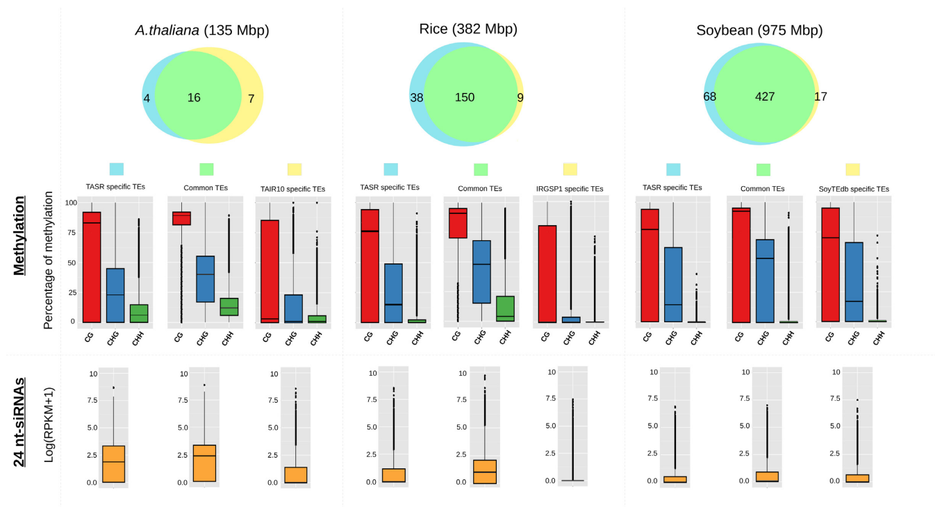
Figure 3. Comparison of the percentage of methylation and 24 nt-siRNAs densities between TEs annotated using TASRs and the public TE annotation in Arabidopsis , rice and soybean.
