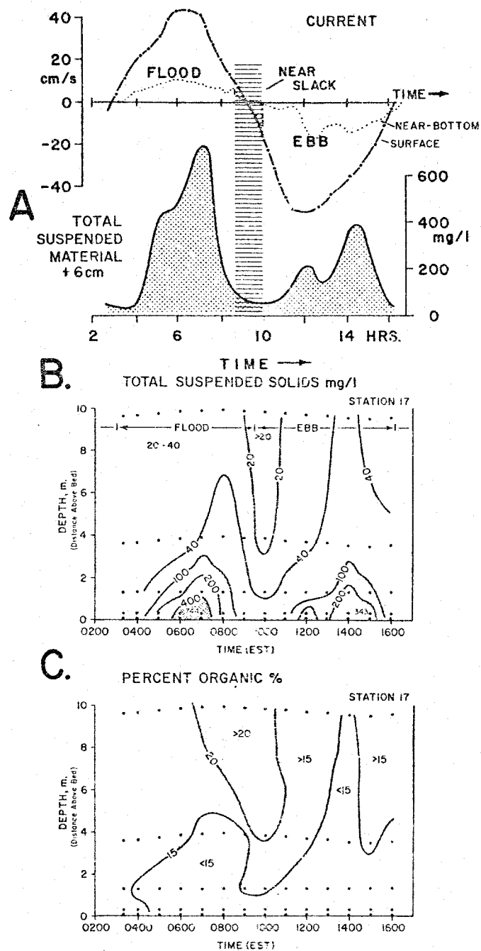
Figure 10. Temporal variation of total suspended material (solids)(B) and percent organic content with depth above the bed (C); anchor station 17, April 30, 1980.
