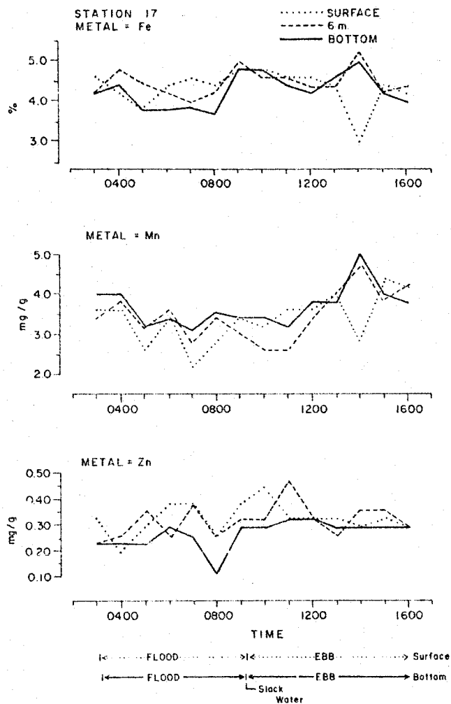
Figure 13. Temporal variation of Fe, Mn and Zn over a tidal cycle at station 17, northern Bay, April 30, 1980.
