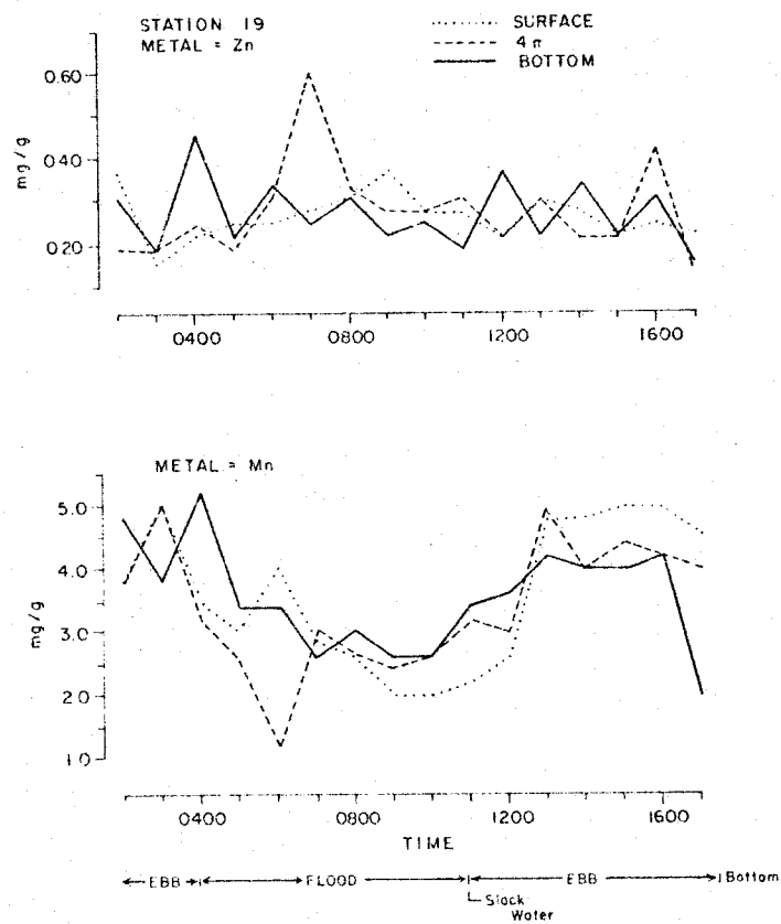
Figure 16. Temporal variation of Zn and Mn over a tidal cycle at station 19, April 29, 1980.
