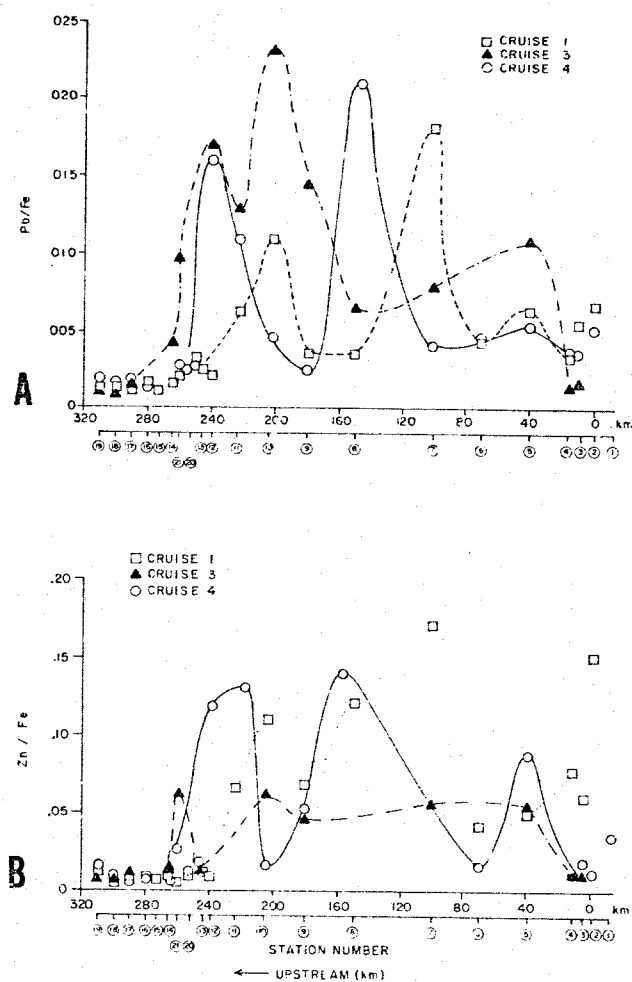
Figure 21. Metal-Fe ratios of mid-depth suspended matter along the Bay length; (A) Pb-Fe; (B) Zn-Fe.
