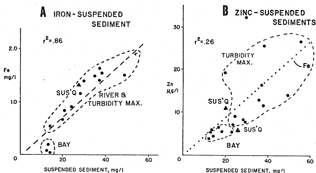
Figure 8. Variation of metal content with total suspended sediment material through a range of conditions from Susquehanna River water through the turbidity maximum zone and partly saline reaches of the northern Bay: A. Iron; B. Zinc; dotted line shows the trend of iron for comparison. Data from near-bottom samples of cruises 5 and 6, April-May, 1980.
