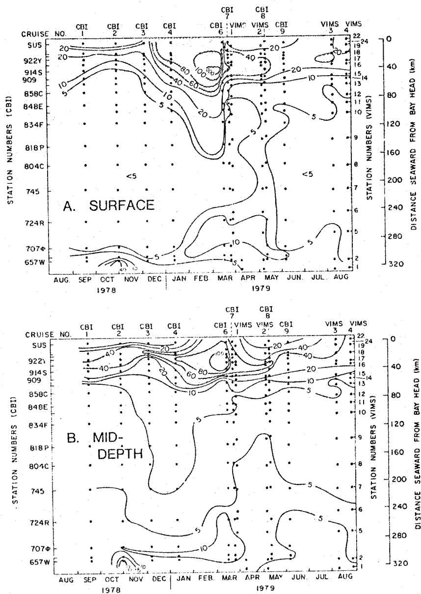
26. Distribution of total suspended material along the Bay axis from August 1978 through August 1979: (A) surface; (B) mid-depth. Zone of the turbidity maximum, shaded.
