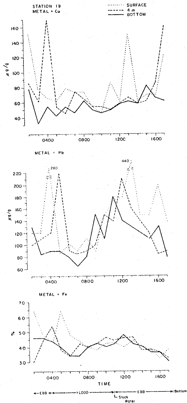
Figure 15. Temporal variation of Cu, Pb and Fe over a tidal cycle at station 19, April 29, 1980.
