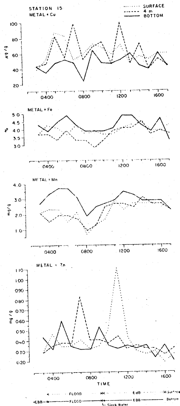
Figure 12. Temporal variation of Cu, Fe, Mn and Zn over a tidal cycle at station 15, northern Bay, May 1, 1980.
