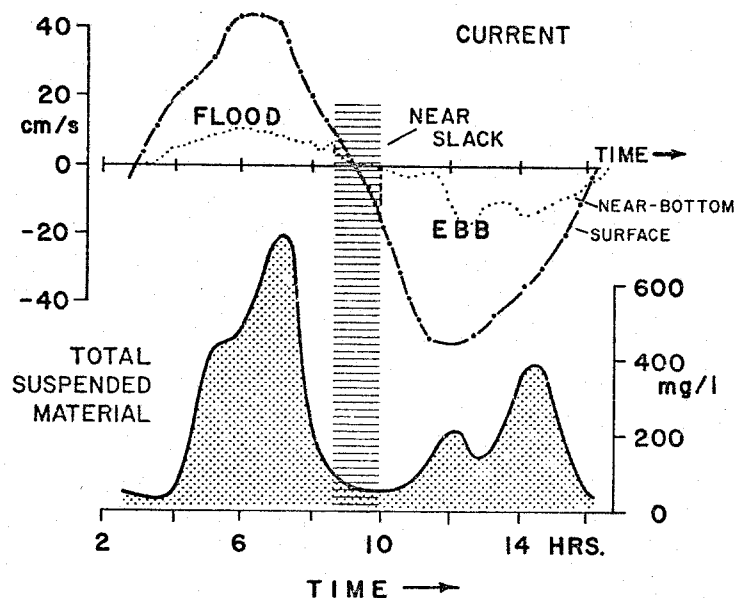
Figure 9. Temporal variation of current velocity and total suspended material at 30 cm above the bed, anchor station 17, April 30, 1980.
