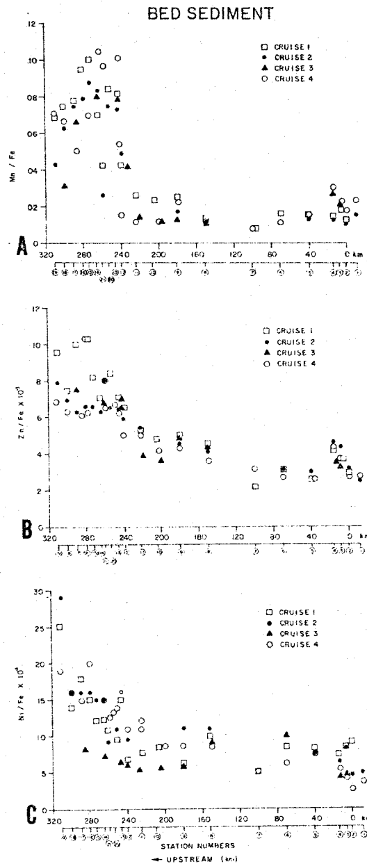
Figure 19. Metal-Fe ratios of bed sediment along the Bay length; (A) Mn/Fe; (B) Zn/Fe; (C) Ni/Fe.
