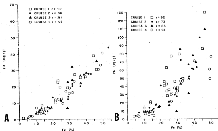
Figure 18. Metal-metal relationships for bottom sediment samples including fluid mud for cruises 1-4; (A) Zn-Fe; (B) Pb-Fe.
