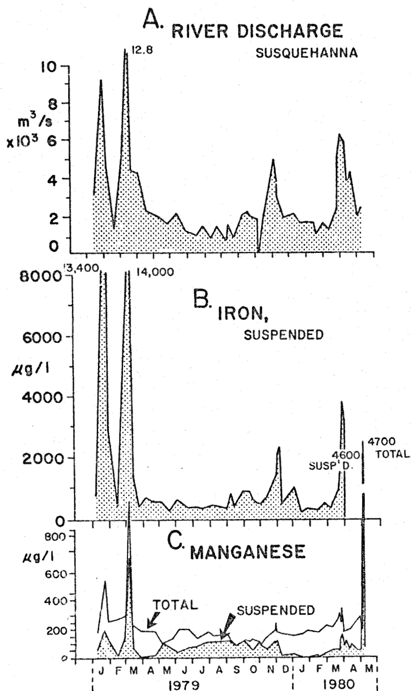
Figure 24. Temporal variations of: (A) Susquehanna River inflow at Conowingo; (B) Iron concentrations; and (C) Mn concentration during 1979-80. Data from U.S.G.S. (23).
