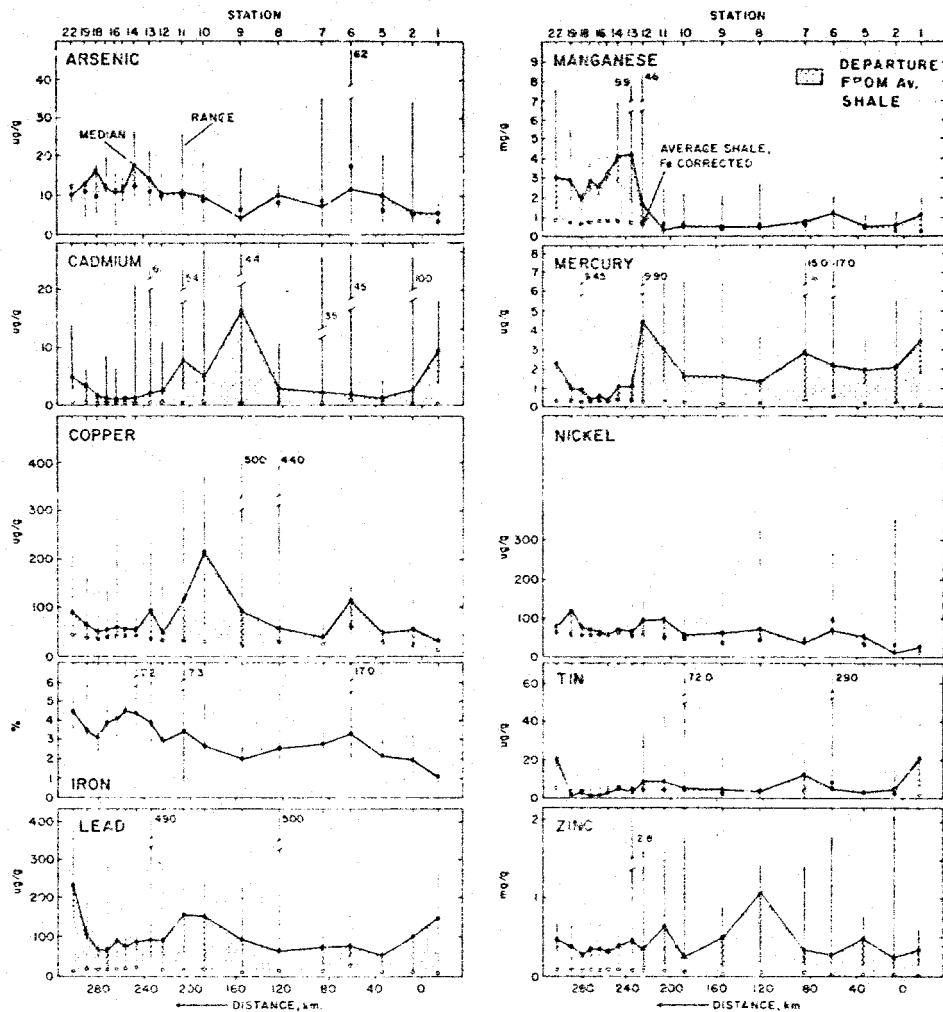
Figure 7. Distribution of metal content in near-bottom suspended material with distance along the Bay axis. Median values and range of concentrations from all available observations of this project. Shaded zone indicates magnitude of departure between median values and mean values for Fe-corrected average shale, open circles.
