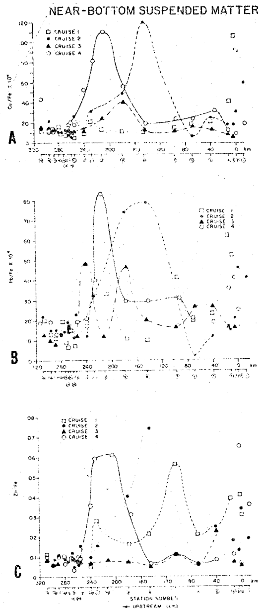
Figure 20. Metal-Fe ratios of near-bottom suspended matter along the Bay length; (A) Cu/Fe; (B) Pb/Fe; (C) Zn/Fe.
