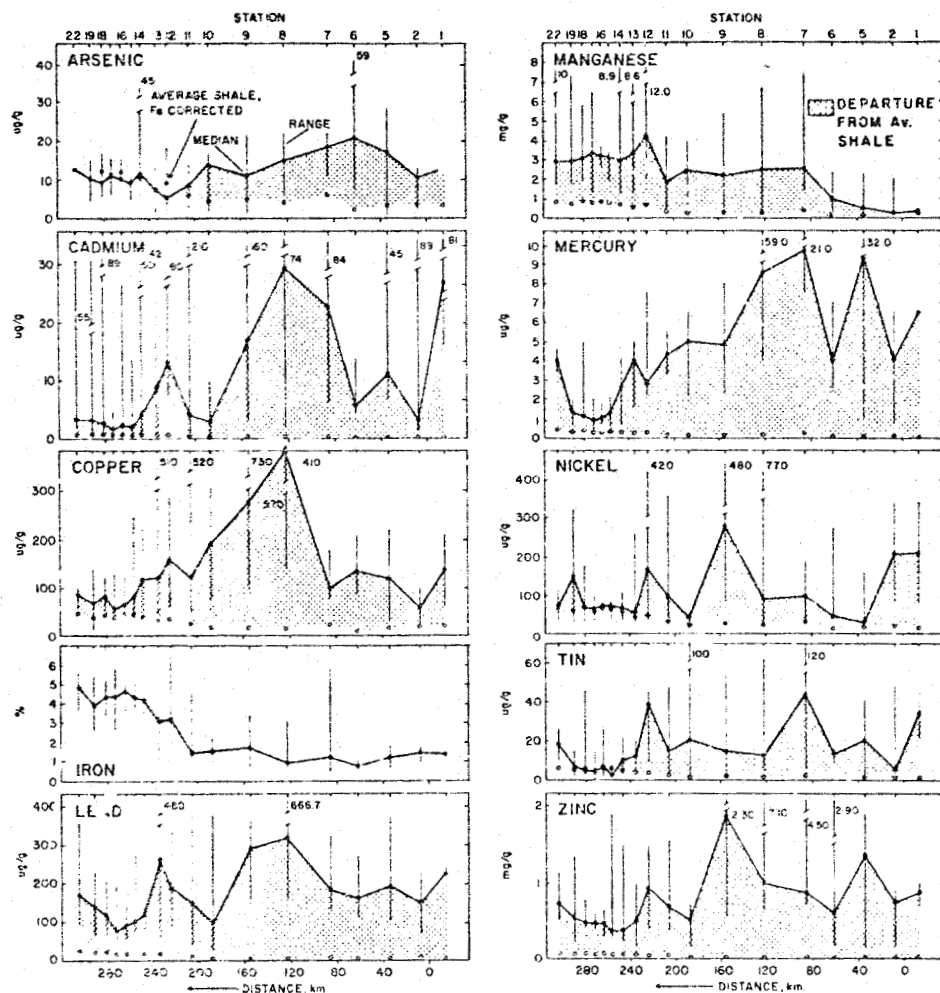
Figure 5. Distribution of metal content in surface suspended material with distance along the Bay axis. Median values and range of concentrations from all available observations of this project. Shaded zone indicates magnitude of departure between median values and mean values for Fe-corrected average shale, open circles.
