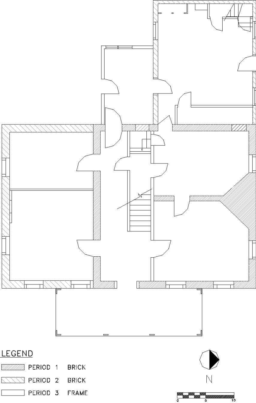
Figure 1: Jehu M. Reed House, first floor plan.
