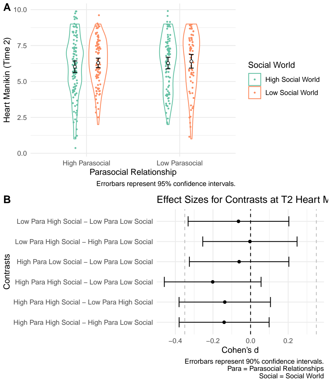
Figure 6.3: Study 3 - Heart Mankin Scores at Time 2 Across Parasocial and Social World Conditions
