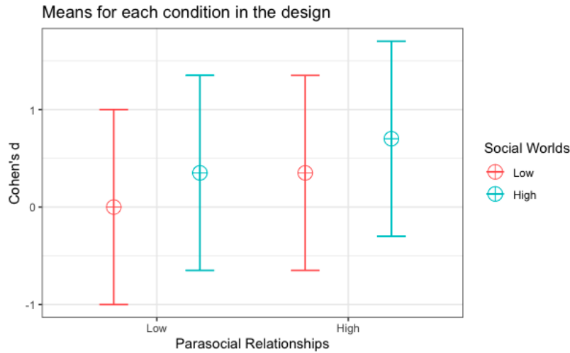
Figure 6.1: Expected Patterns of the Means Used for the Power Analysis for Study 3
