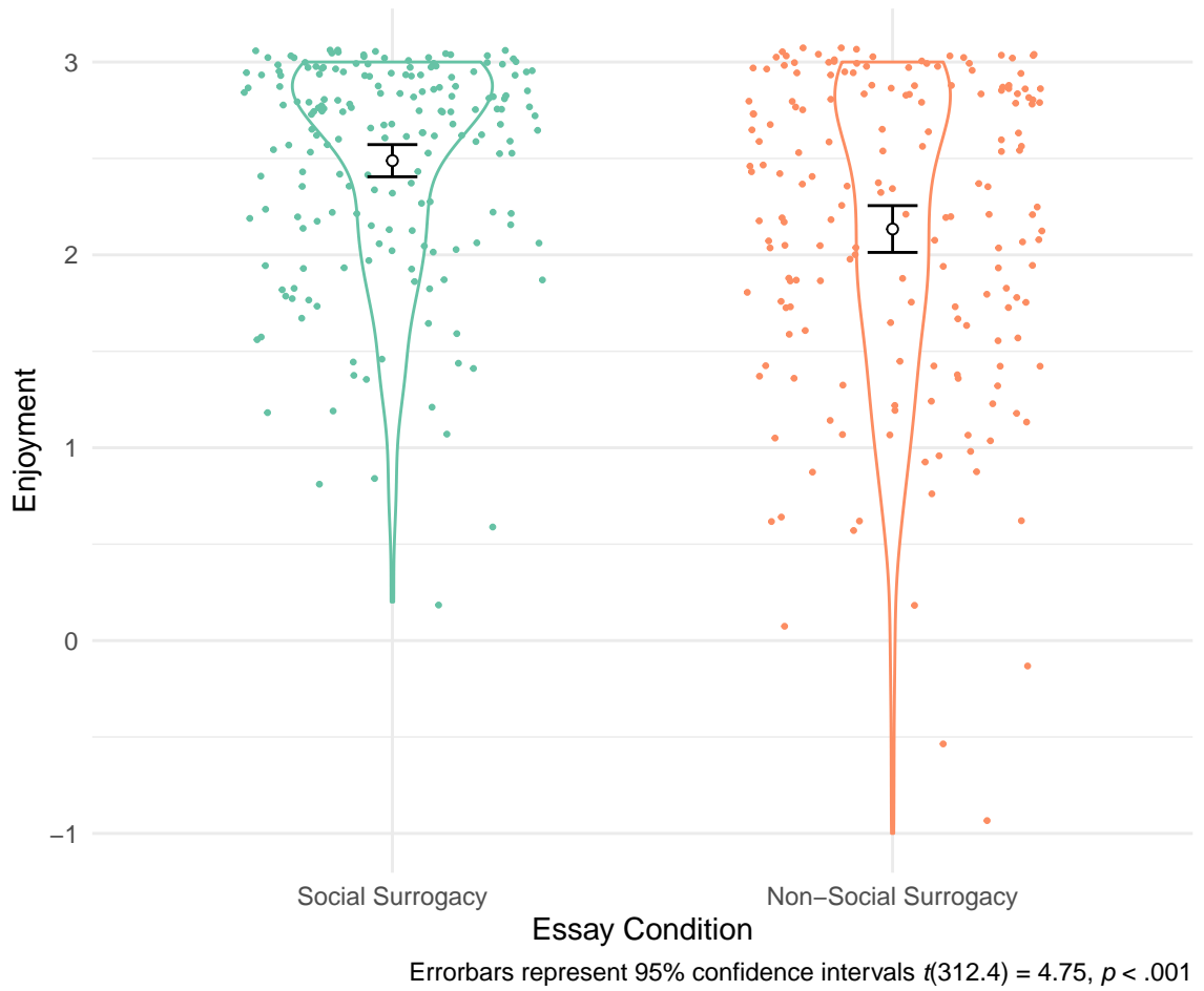
Figure 5.5: Study 2 - Enjoyment across Essay Conditions
