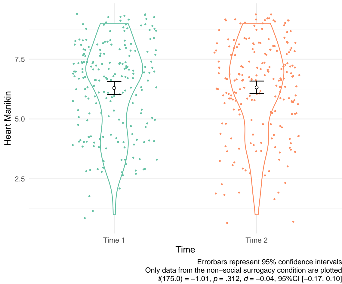
Figure 5.2: Study 2 - Heart Mankin Scores at Times 1 & 2 among the Non-Surrogate Group
