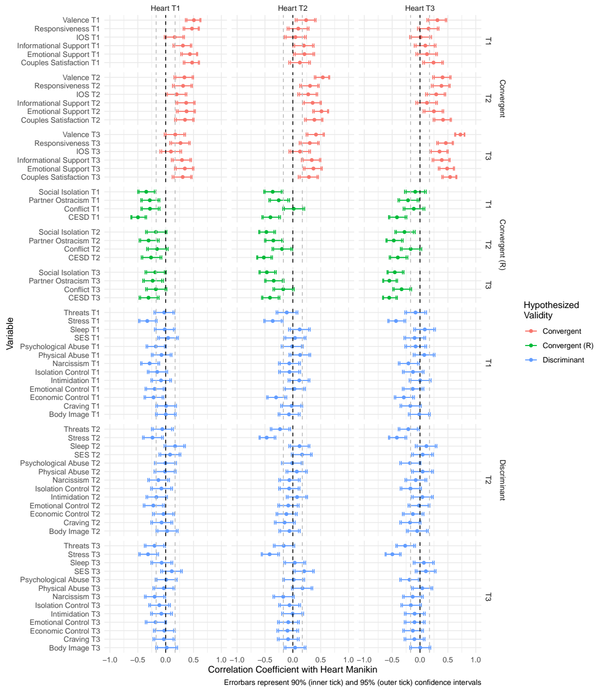
Study 1b (RAIv1): Correlation Coefficients with the Heart Manikin across Visits 1–3
