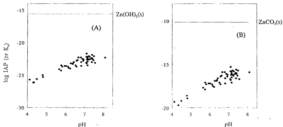
Figure 2. Saturation state of lake waters with respect to \text{Zn}(\text{OH})_2(\text{s}) (A) and \text{ZnCO}_3(\text{s}) (B). IAP is the ion activity product. The horizontal lines correspond to the solubility products.
