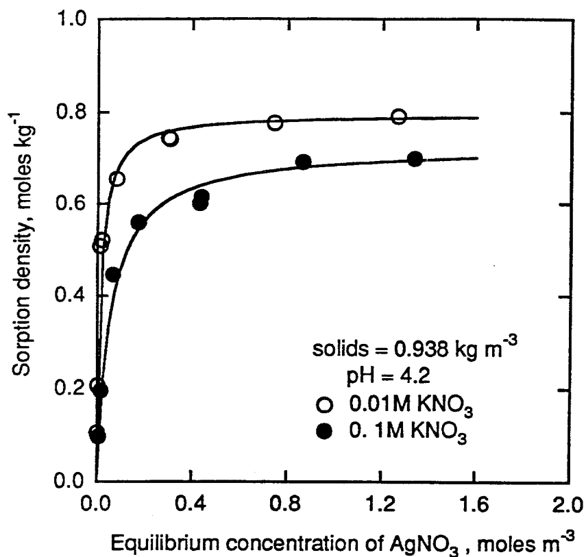
Figure 5. Sorption isotherms at pH 4.2 \pm 0.05 .
