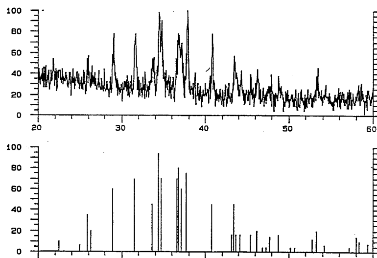
Figure 1b. XRD spectrum of Ag 2 S precipitate compared to Acanthite standard
