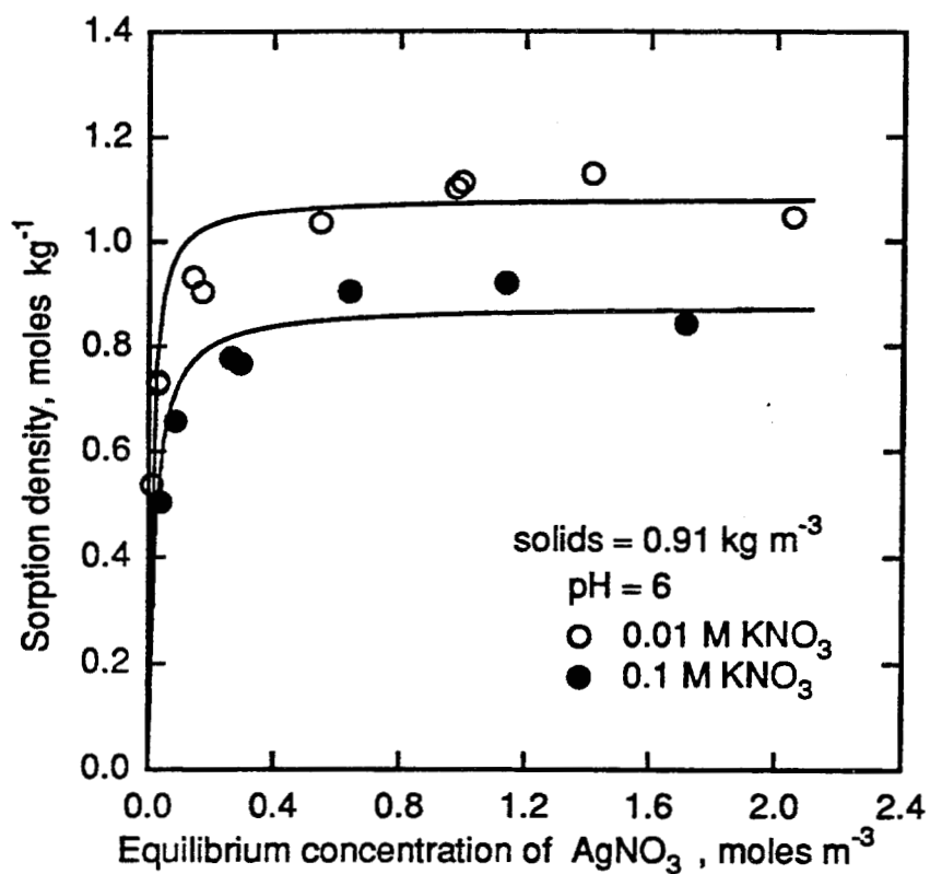
Figure 3. Sorption isotherms at \text{pH } 6 \pm 0.15 .
