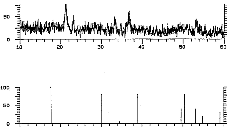
Figure 1a. XRD spectrum of FeS precipitate compared to Mackinawite standard
