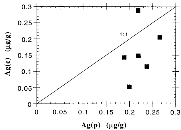
Figure 5. Ag concentrations in colloidal matter ( \text{Ag(c)} ) plotted as a function of Ag concentrations in suspended matter ( \text{Ag(p)} ).
