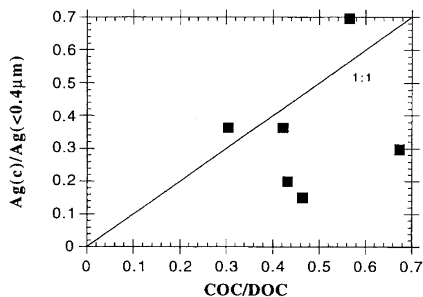
Figure 6. Fraction of colloidal silver, [\text{Ag(c)}]/[\text{Ag}(\leq 0.4\mu\text{m})] , as a function of the fraction of colloidal carbon, [\text{COC}]/[\text{DOC}] .
