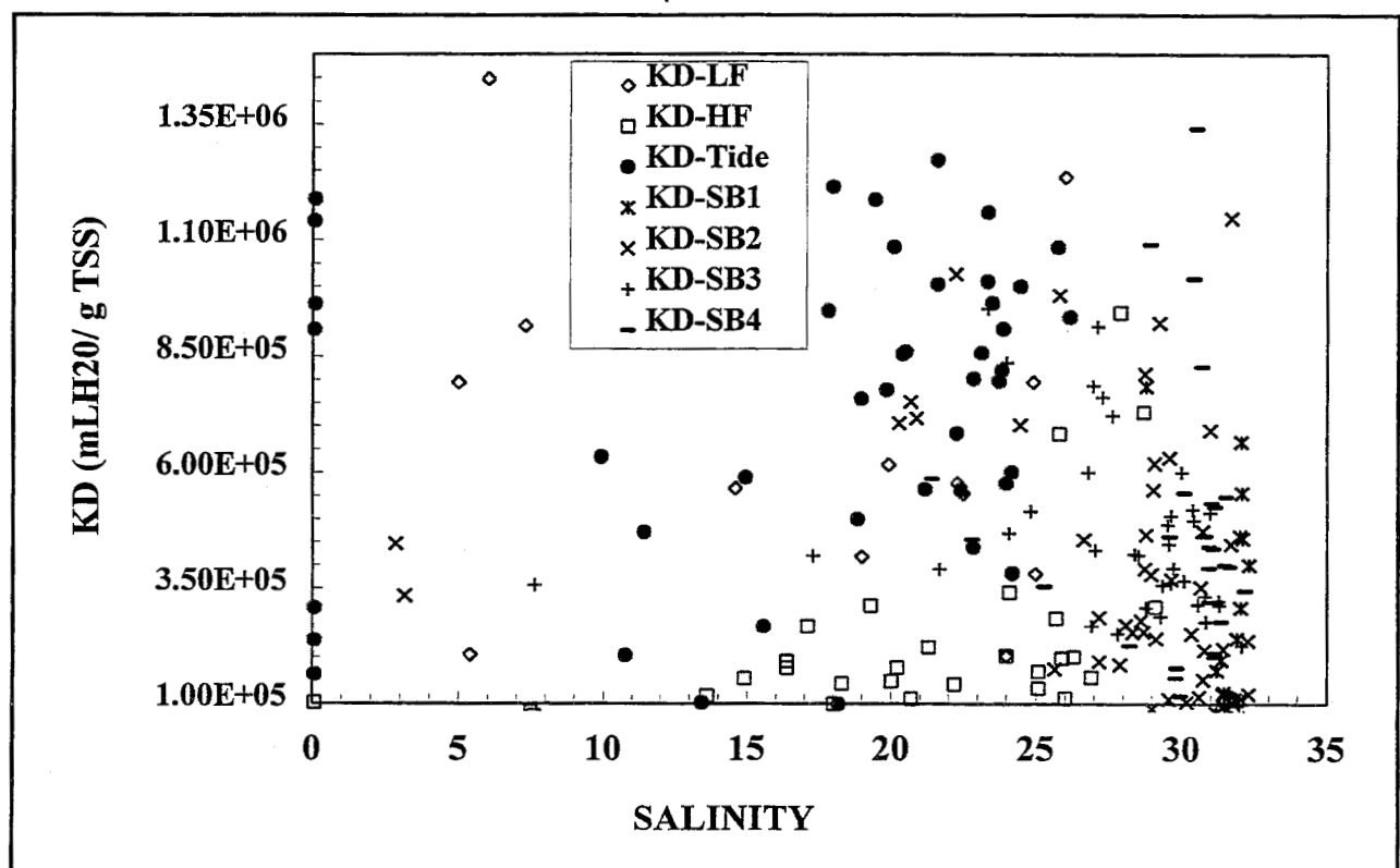
Figure 2. Partitioning coefficient versus the salinity of each sample all surveys.
