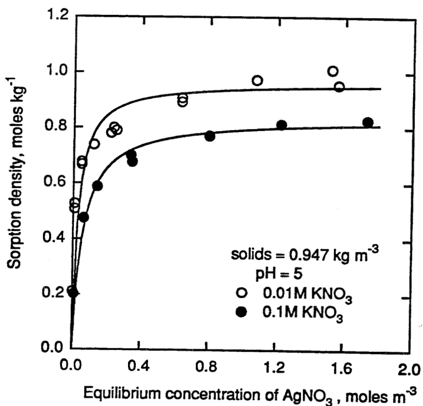
Figure 4. Sorption isotherms at \text{pH } 5.0 \pm 0.1 .
