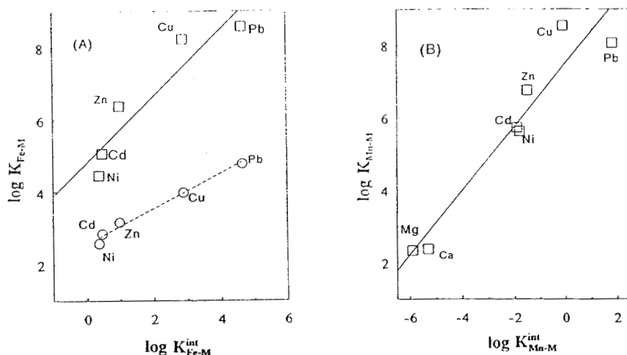
Figure 4. Correlations between log K Fe-M and log K Fe-M int (A) or between log K Mn-M and log K Mn-M int (B). (□) and (○) are for McFarlane (pH 7.4) and Clearwater (pH 4.8) lakes, respectively.
