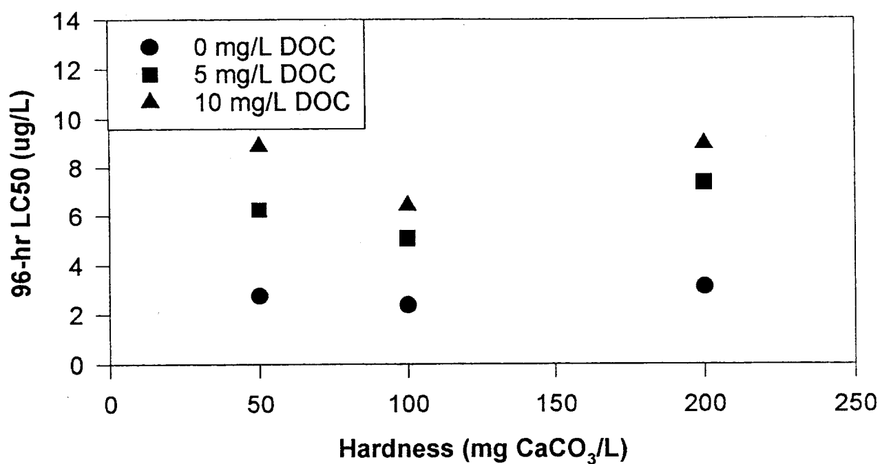
Figure 5. Effect of Hardness on Acute Silver Toxicity to Larval Fathead Minnows, at 3 Levels of DOC and 3 mg/L Chloride.
