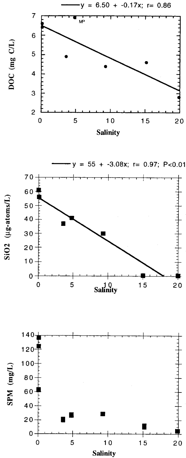
Figure 2. a) Dissolved organic carbon, DOC, b) dissolved SiO 2 and c) suspended particulate matter, SPM, across a salinity transect in Galveston Bay, taken in May 1994. MP indicates a sample from Morgan's Point (see Figure 1).
