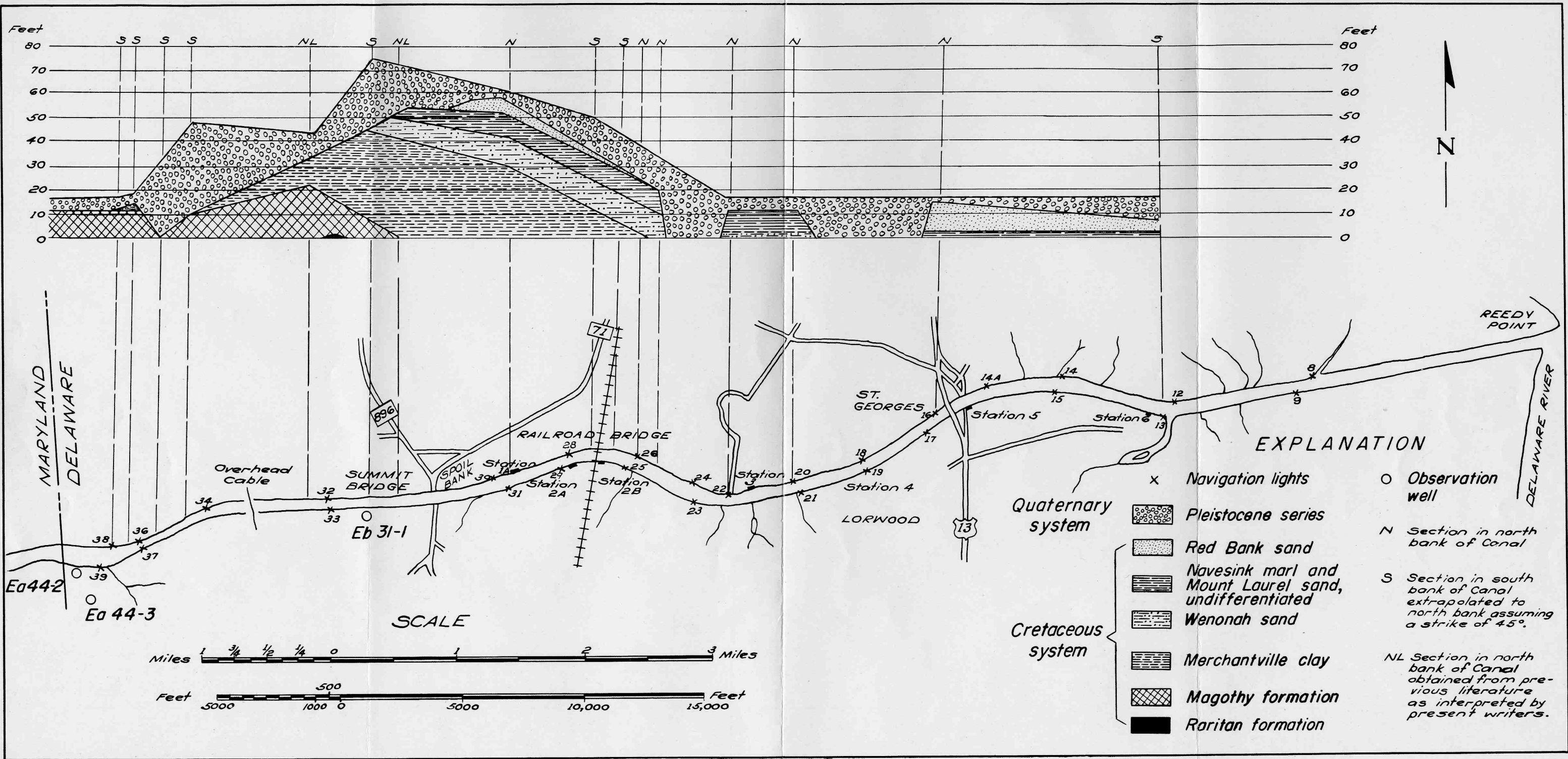
Plate 7.--Geologic cross section of the outcrop of Cretaceous rocks and Pleistocene deposits along the Chesapeake and Delaware Canal.
